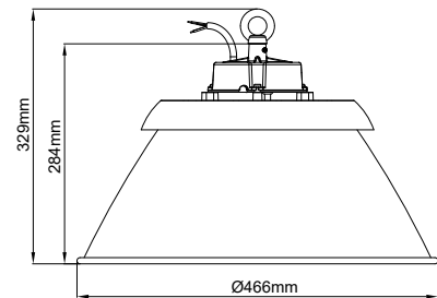
Tall Reflector
