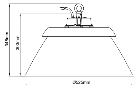
Tall Reflector
