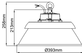
Universal Reflector
